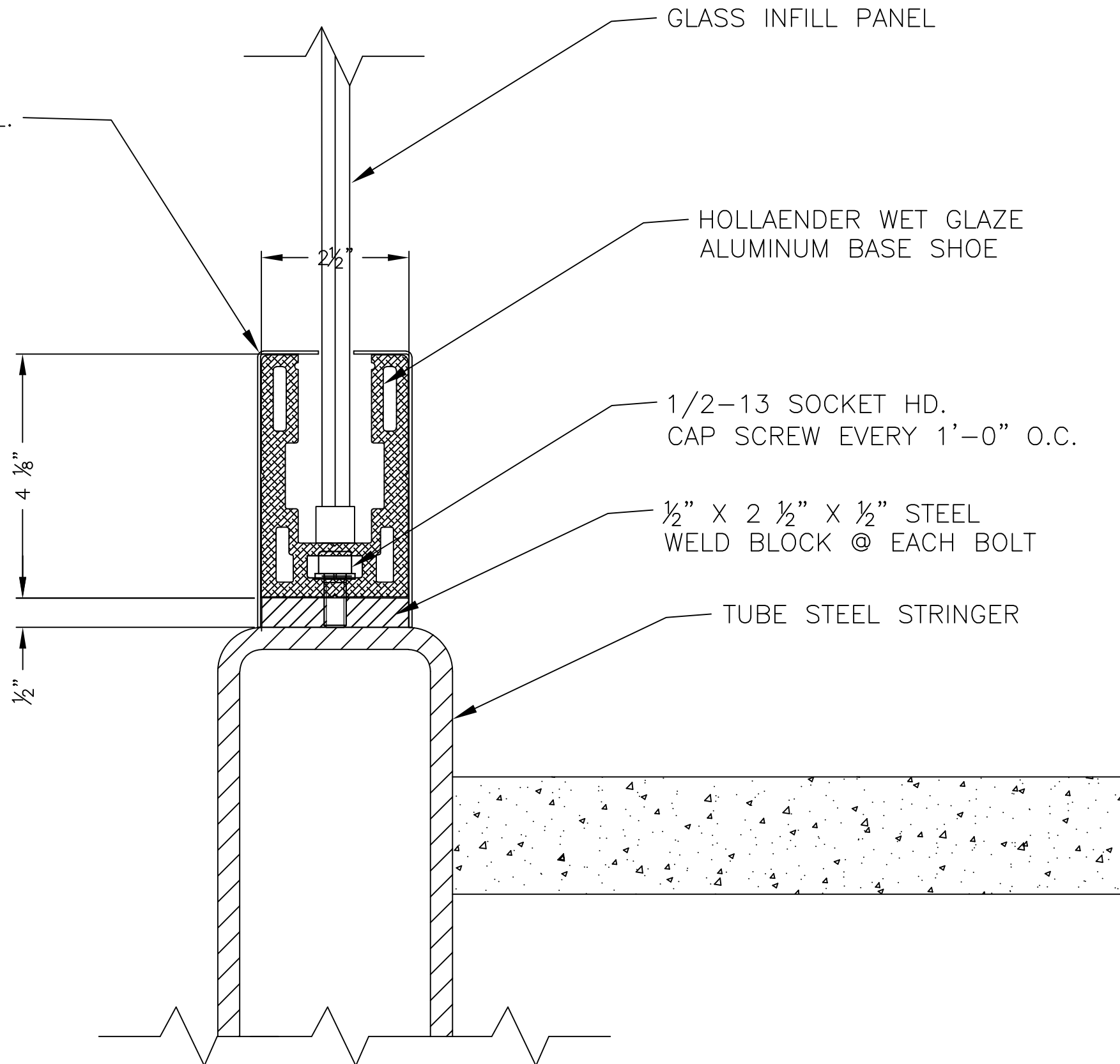
WET GLAZE BASE SHOE W/ WELD BLOCK TOP MOUNTED TO TUBE STRINGER
