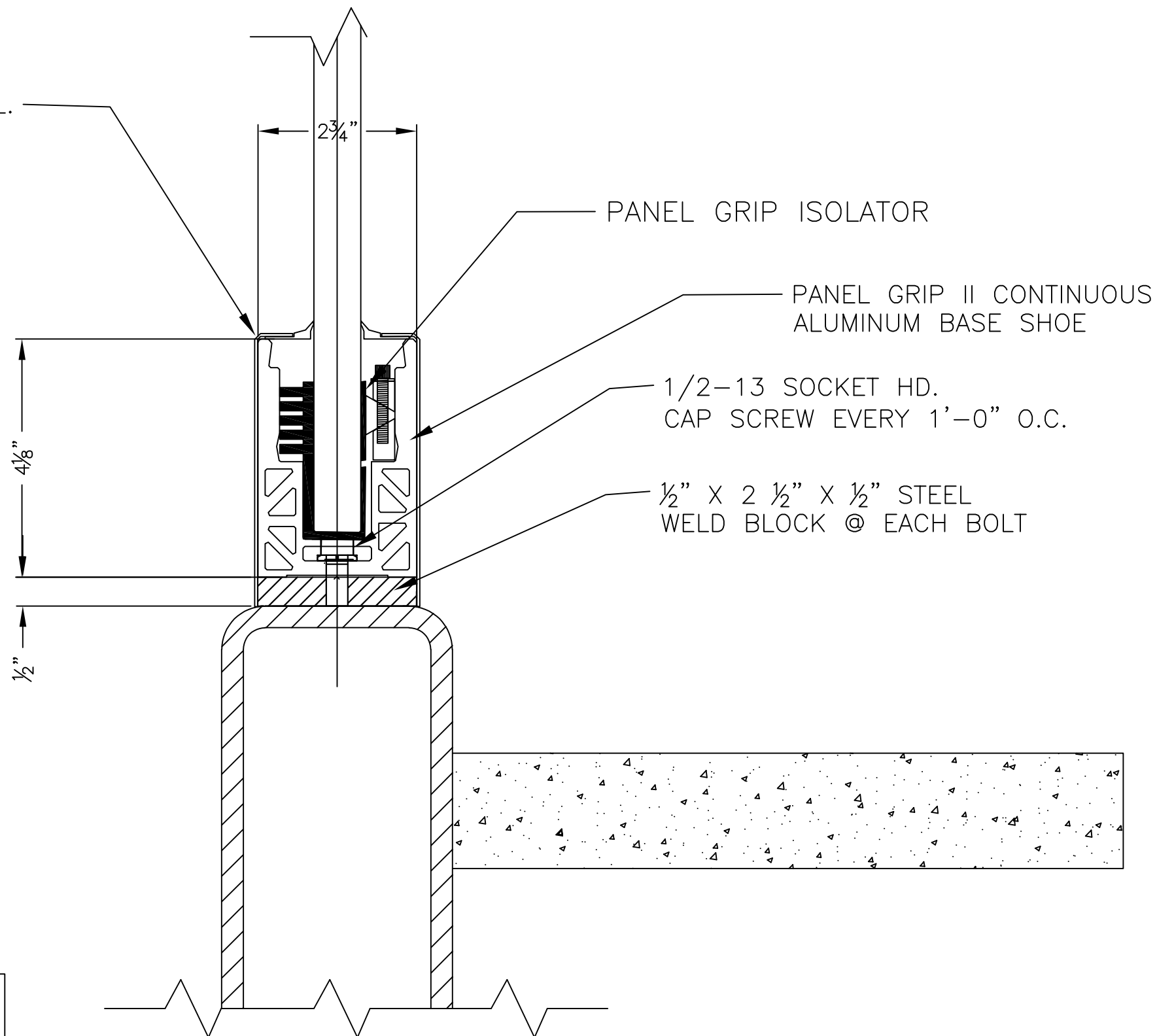
PANEL GRIP II DRY SET BASE SHOE W/ WELD BLOCK TOP MOUNTED TO TUBE STRINGER
