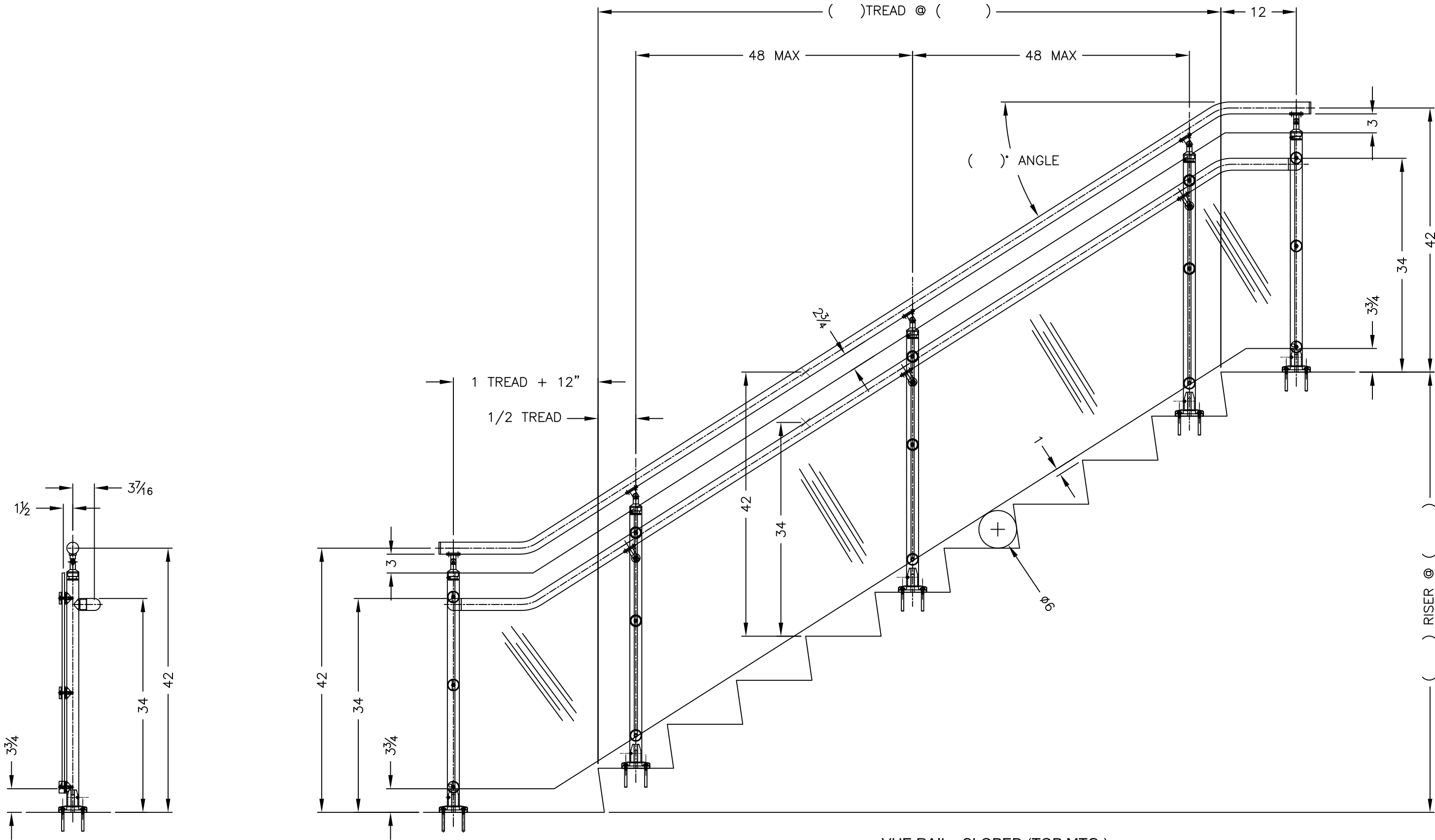
VUE RAIL - SLOPED (TOP MTG.) GUARD RAIL w/ GRAB RAIL
